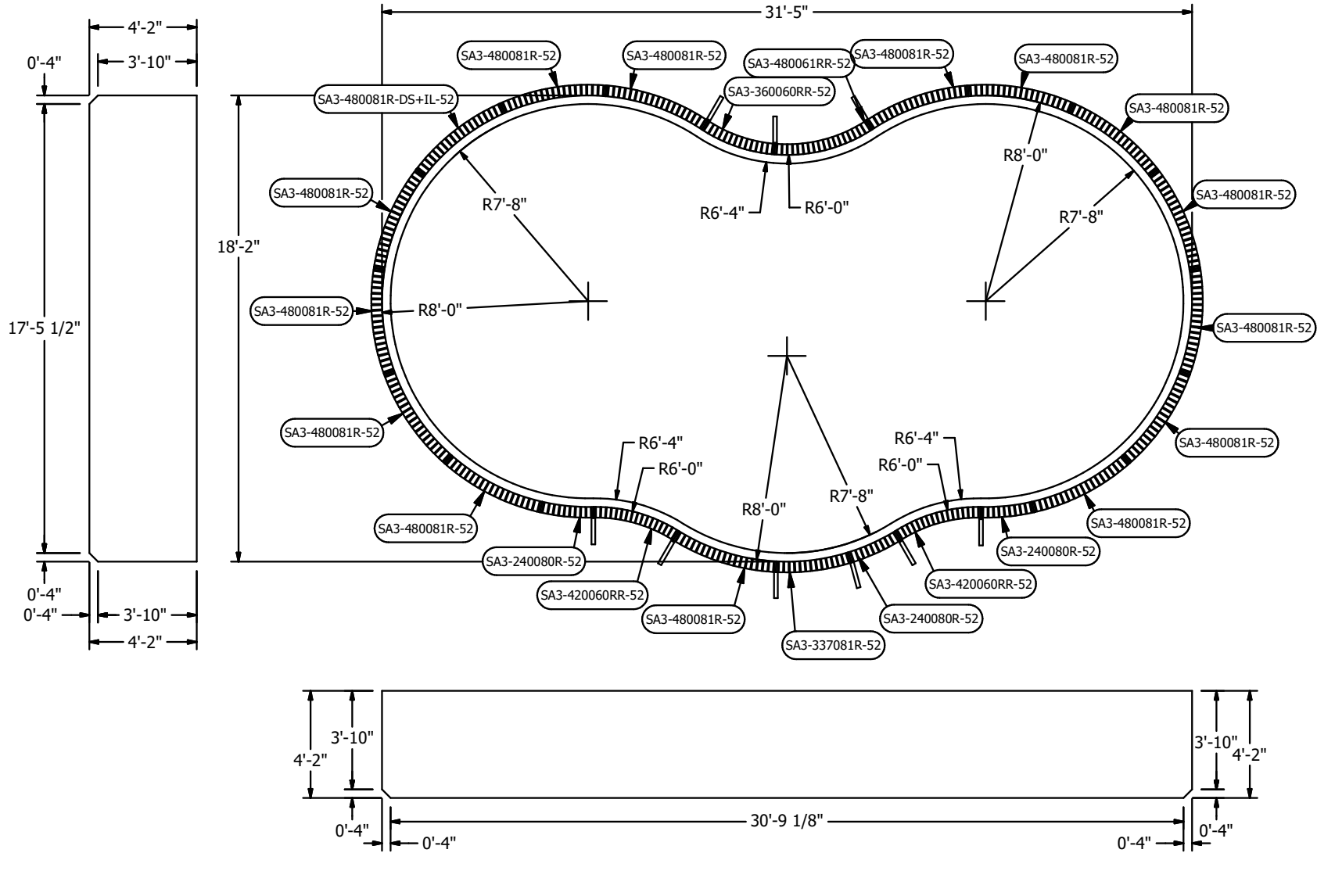
SA3-BTBR-Z (SIDE PROFILE)
